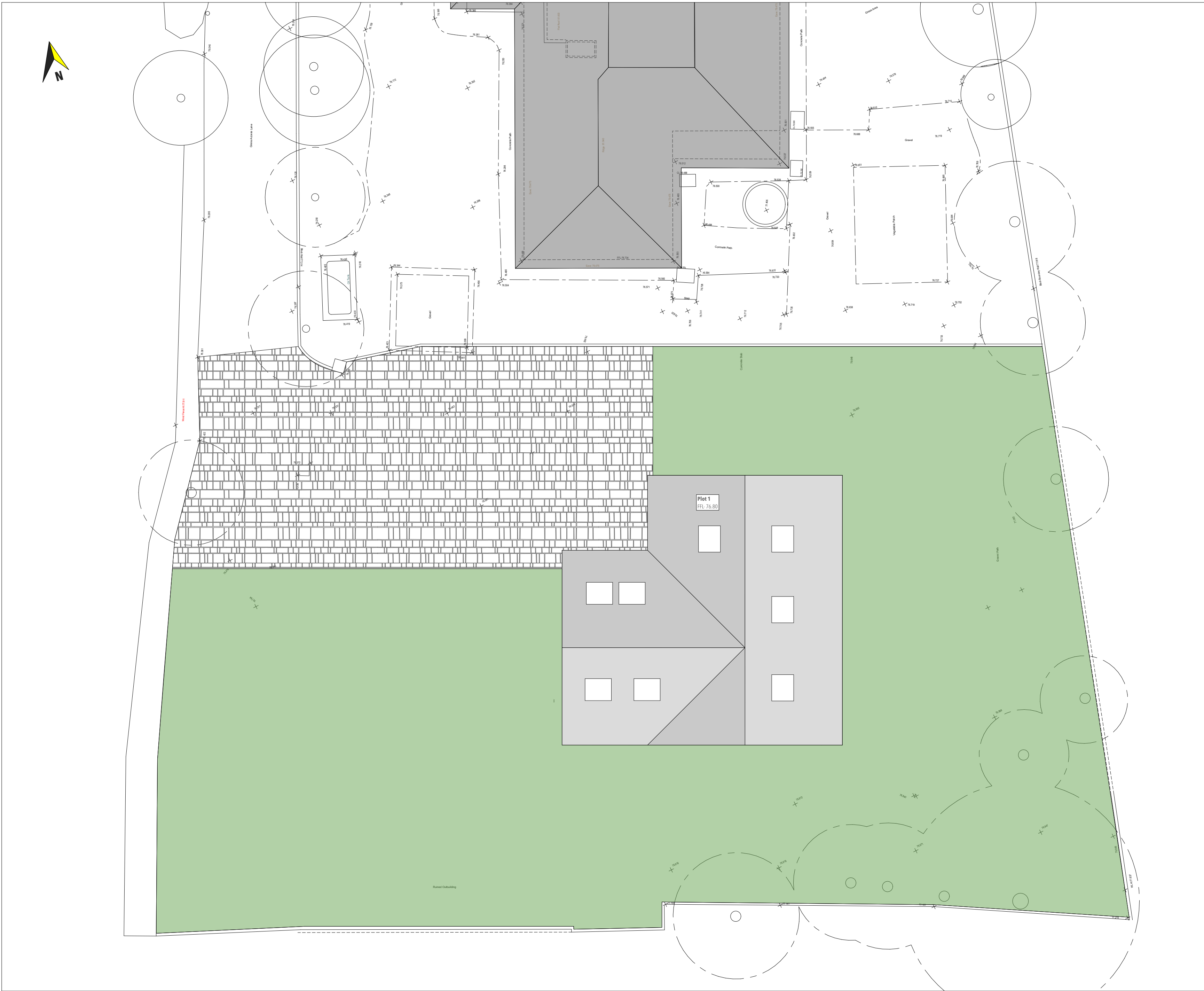
Proposed Site Layout 1:100
